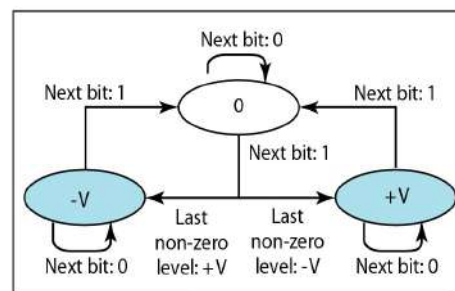
c. Transition states
